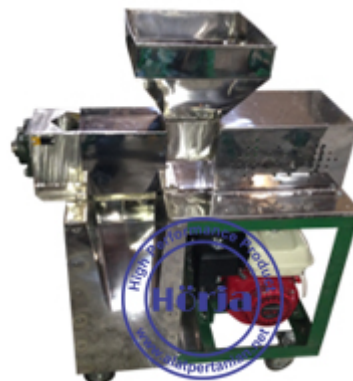
Capacity (kg) : 500-1000 kg/hour (width) : 450 mm (height) : 1000 mm (power) : 1.5 Kw
